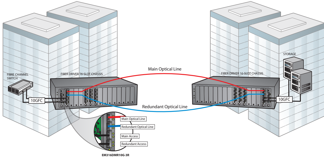
Figure 2: Redundant Converter/Repeater/Transponder
