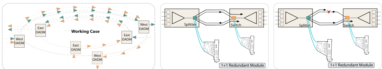
Link protected network operating with unbroken redundant link
