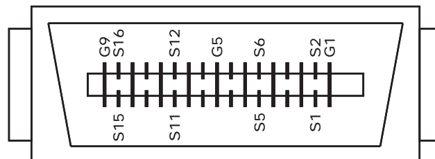
Front-View CX4 Connector
