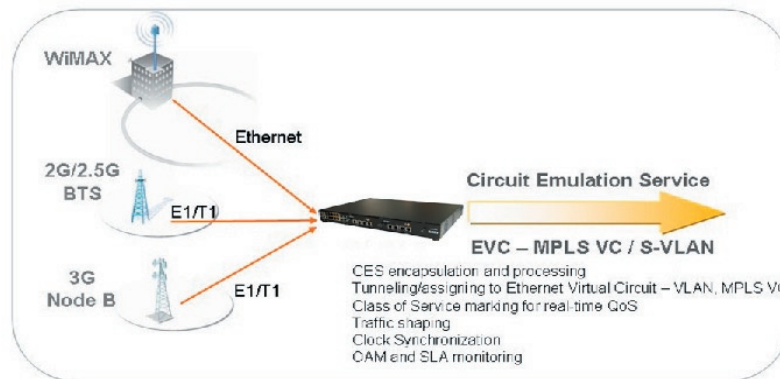
OS910-M leverages resiliency, OAM, QoS & Multi-Service capabilities over Metro Ethernet IP/MPLS transport
